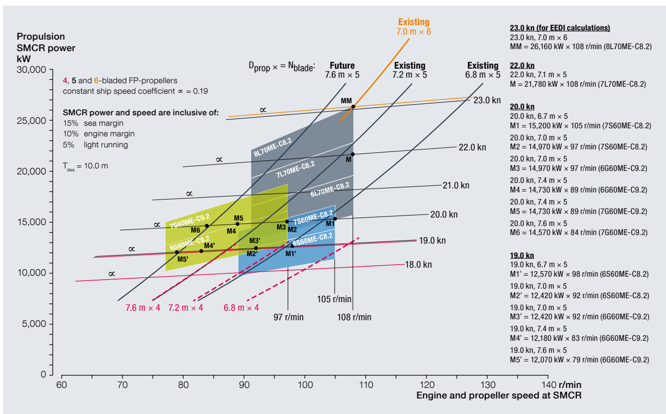
Fig. 4: Different main engine and propeller layouts and SMCR possibilities (M1, M2, M3, etc. for 20.0 knots and M1', M2', M3', etc. for 19.0 knots) for a 2,500 teu container ship operating at 20.0 knots and 19.0 knots, respectively
