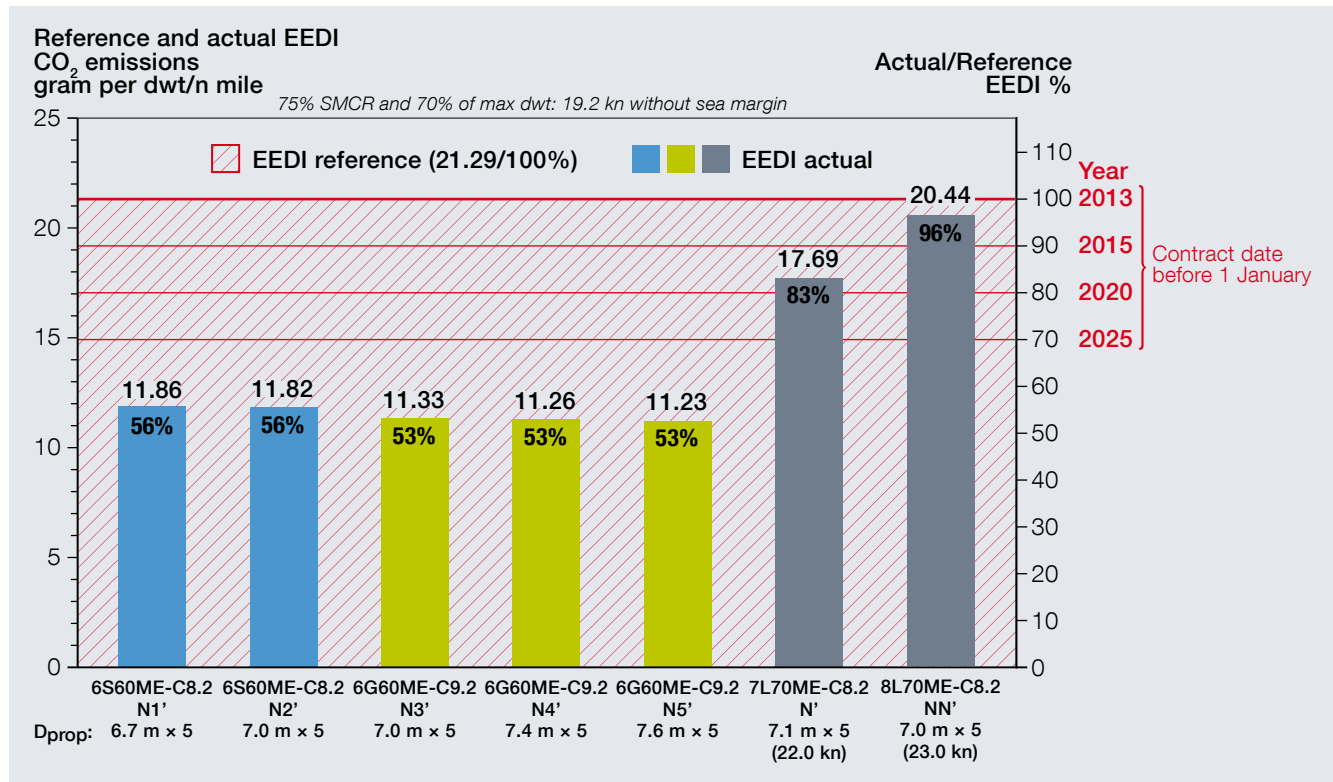
Fig. 14: Reference and actual Energy Efficiency Design Index (EEDI) for 19.0 knots
